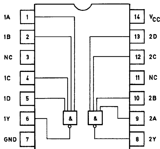
Dual 4-input Nand gates with open collector outputs
