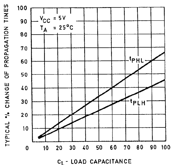
Propagation times Vs. load capacitance
