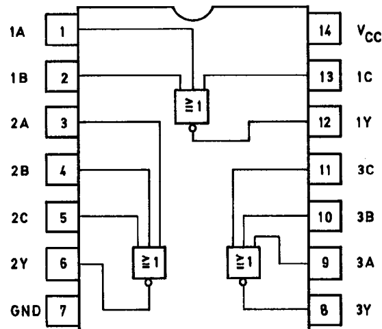
Three 3-input positive-Nor gates
