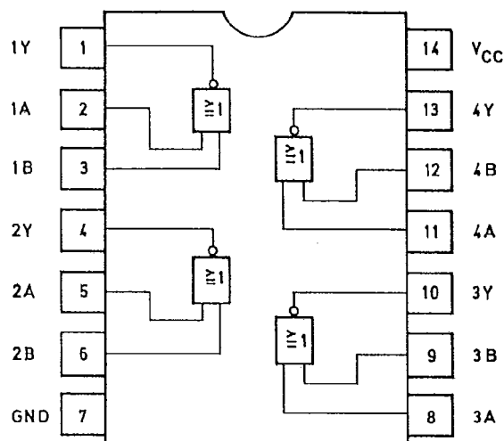
Quad 2-input Nor buffers
