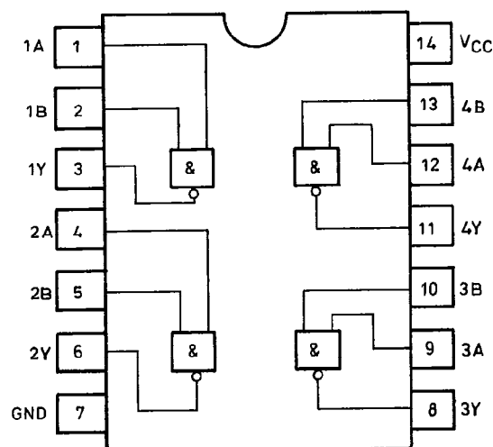
Quad 2-input Nand buffers
