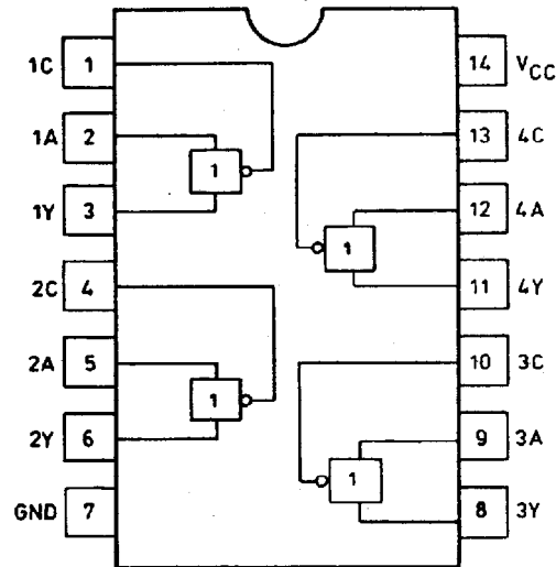
Four bus buffer gates with three level output
