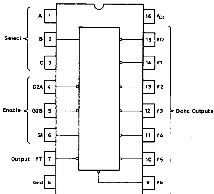
3-to-8 Line decoders/demultiplexers
