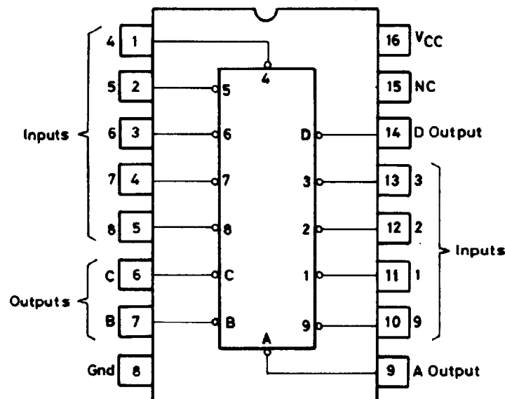
10-line decimal to 4-line BCD priority encoder
