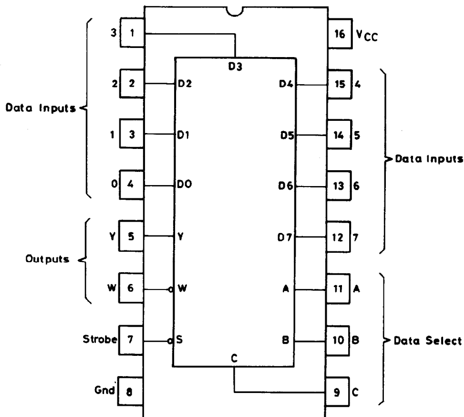
Data selector/multiplexers
