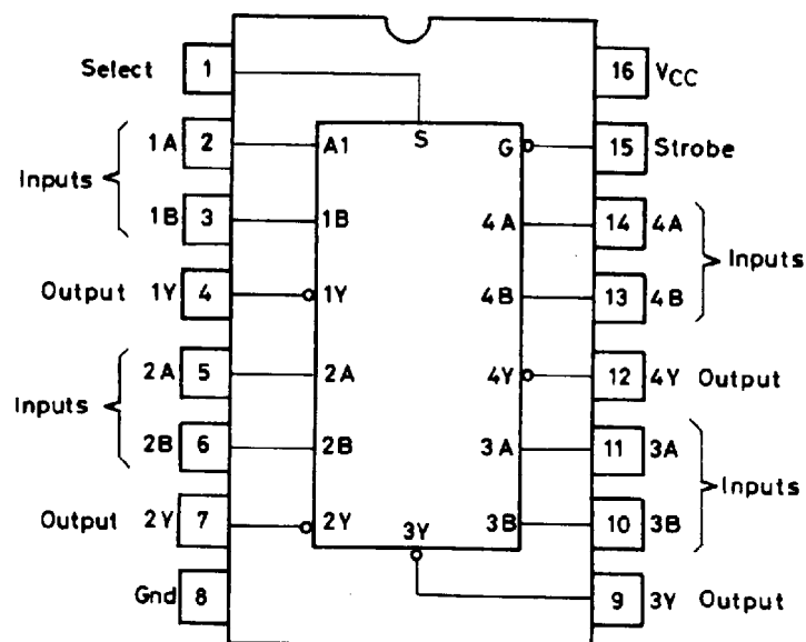
Quad 2-line to 1-line data selector/ multiplexer with inverted outputs
