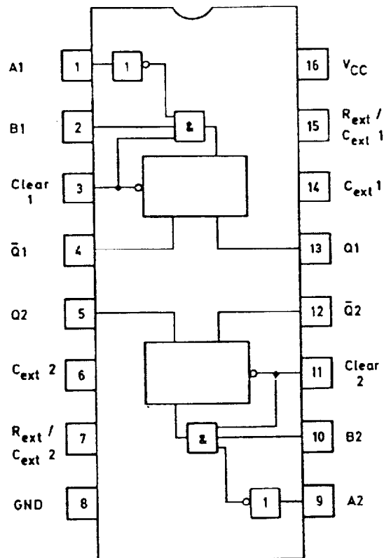
Dual retriggerable monostable multivibrator with clear
