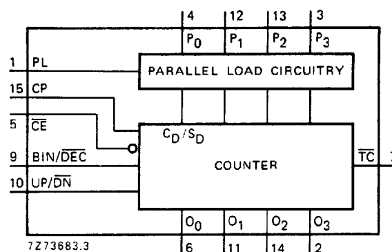
Fig. 3 Functional diagram.
