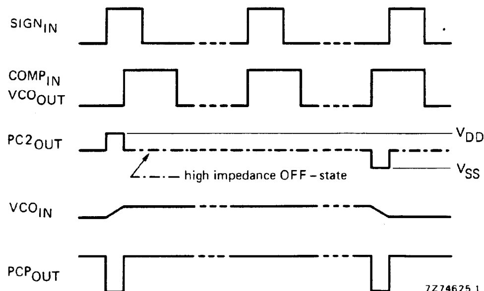
Fig. 3 Typical waveforms for phase-locked loop employing phase comparator 2 in locked condition.
