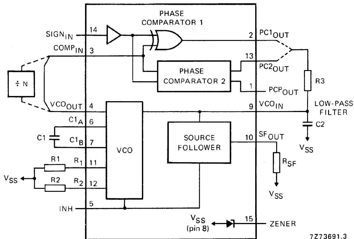
Fig. 5 Functional diagram.
