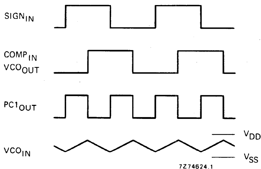
Fig. 2 Typical waveforms for phase-locked loop employing phase comparator 1 in locked condition of f_0 .
