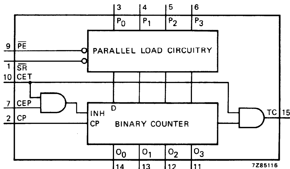
Fig. 2 Functional diagram.
