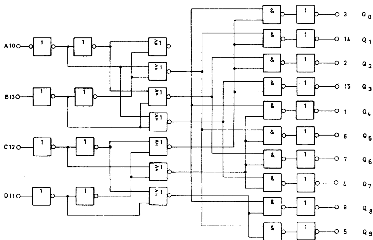
Typical logic diagram
