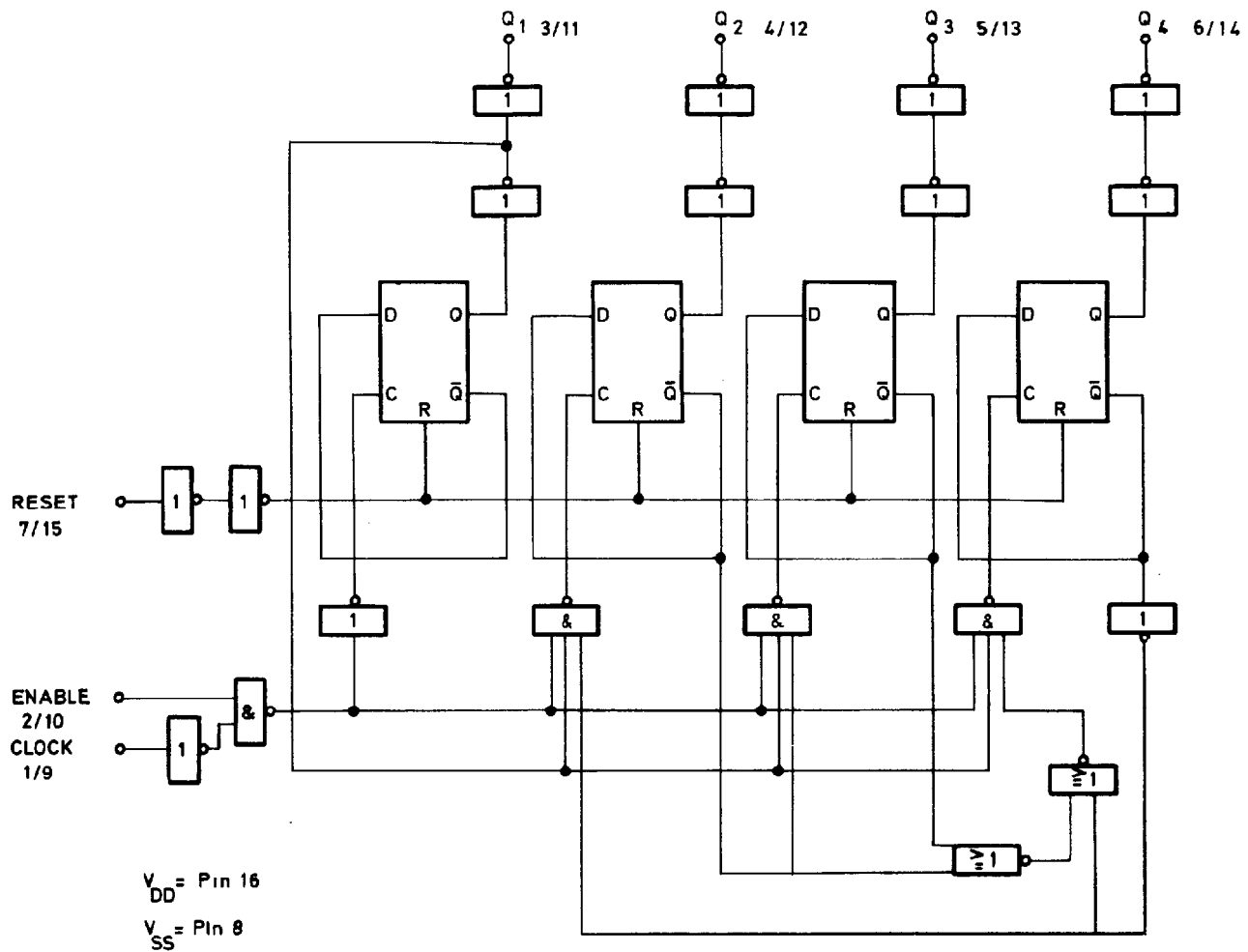
Typical logic diagram
