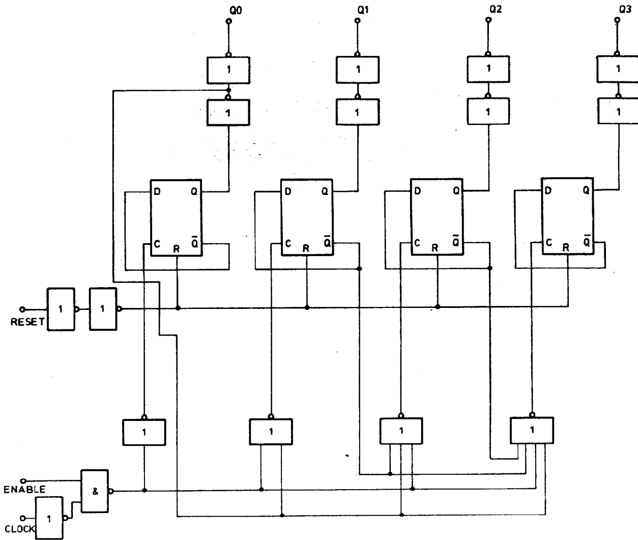
Typical logic diagram
