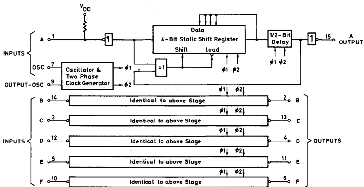
Typical logic diagram
