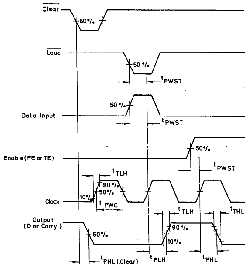
Switching time waveforms
