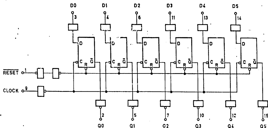
Typical logic diagram
