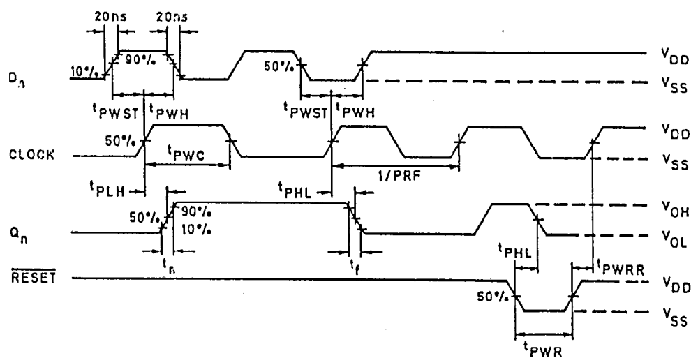
Switching time waveforms
