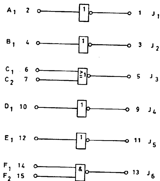
Function block diagram
