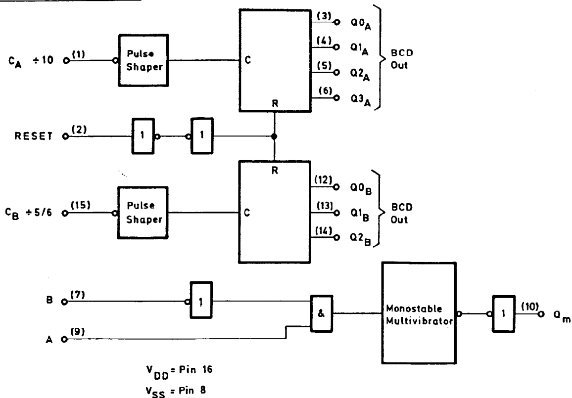
This is a graphic representation not a circuit diagram Figure 2
