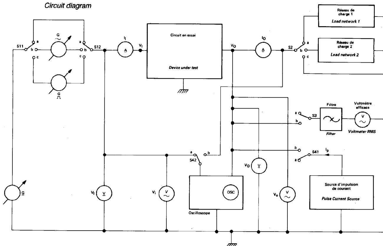
4.0 Schéma Circuit diagram
