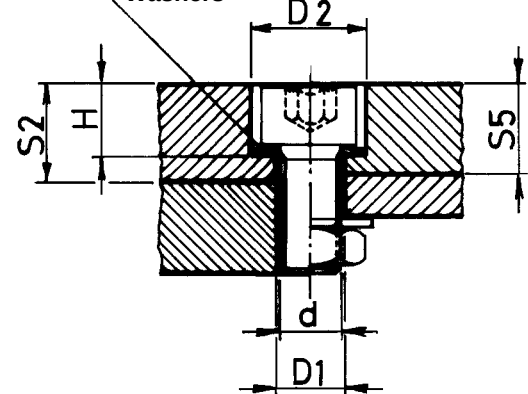
Rosette N 3.400.015 Washers
