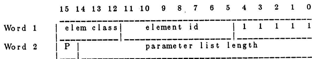
Figure 2. Format of a long-form Command Header.
