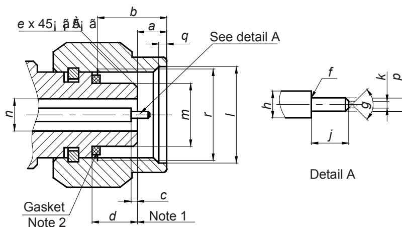
Figure 1 – Connector with pin- centre contact (for dimensions, see Table 1)
