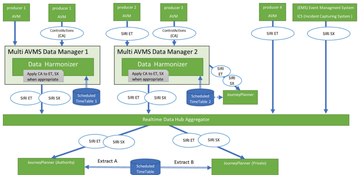
Figure 2 — System with Data Harmonisers feeding a Data Hub (and using control actions)
