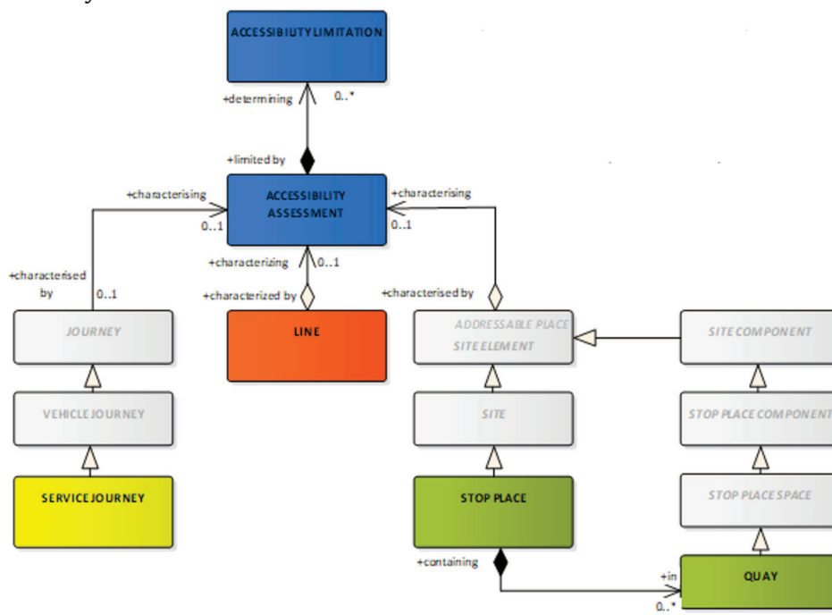
Figure 10 – Accessibility (UML)
