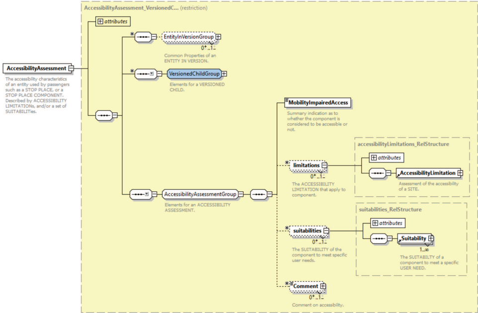
Figure 11 — AccessibilityAssessment - XSD (when used on StopPlace only then valid for all elements of the StopPlace)
