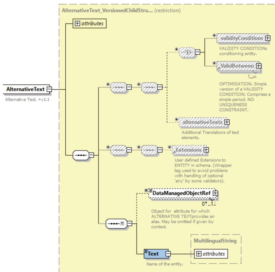
Figure 8 — AlternativeText - XSD
