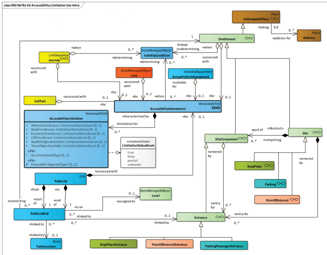
Figure 12 — Accessibility Assessment -Physical Model (UML)
