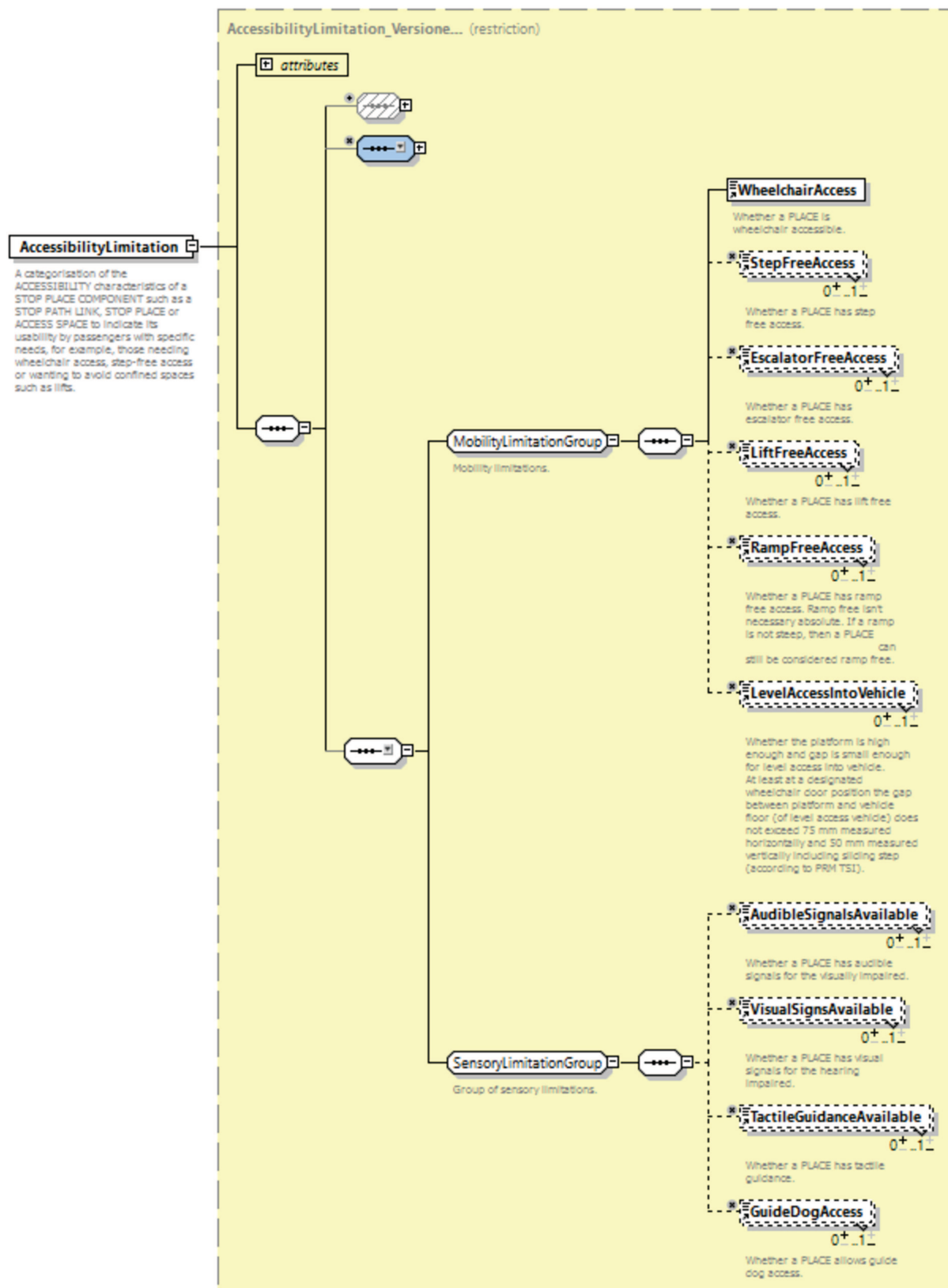
Figure 13 — AccessibilityLimitation - XSD
