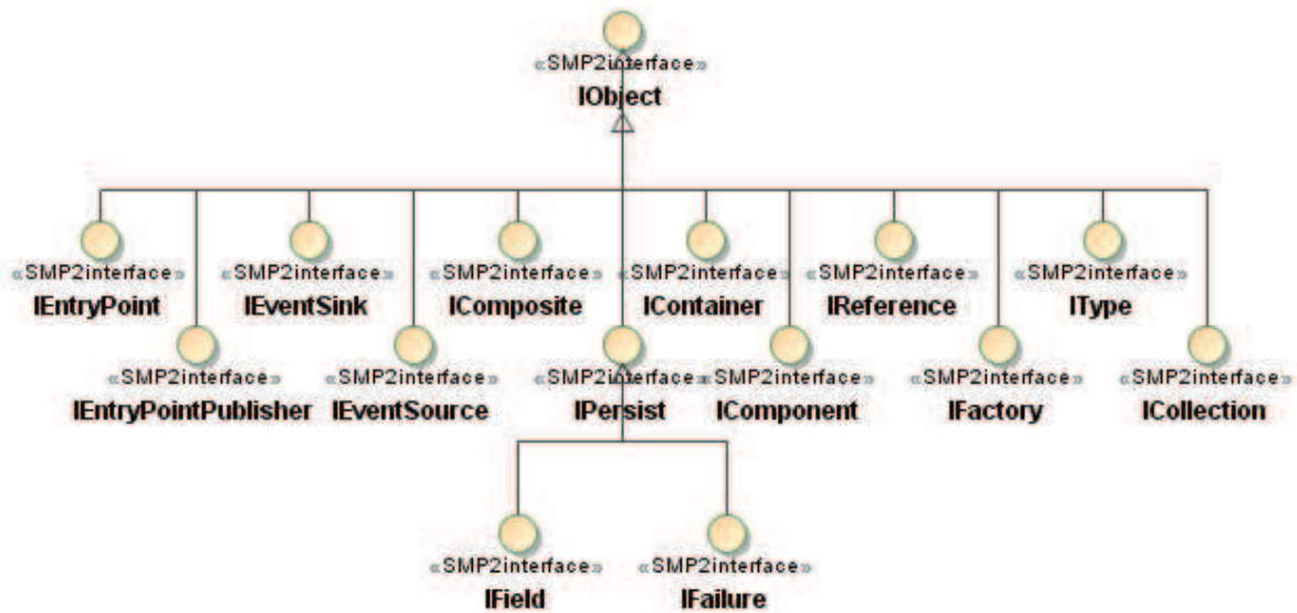
Figure 4-4: Object mechanisms
