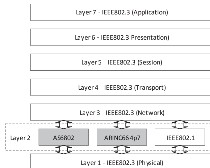
Figure 4-4: Time-Triggered Ethernet Services
