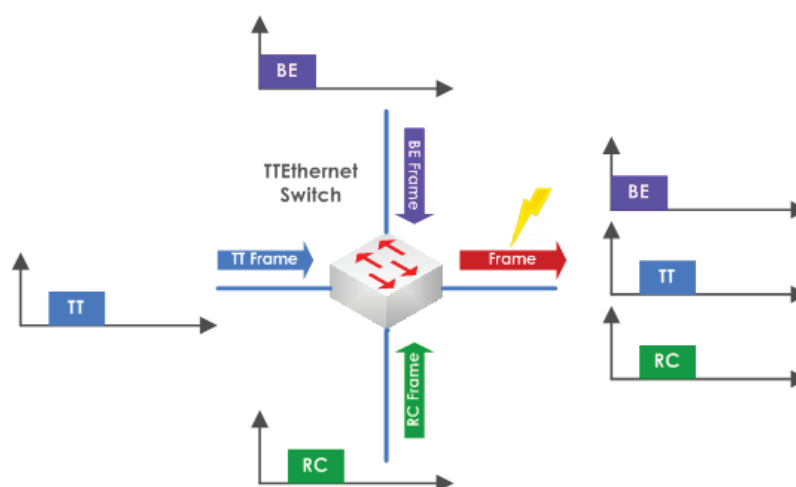
Figure 4-9: Message Processing at the Switch
