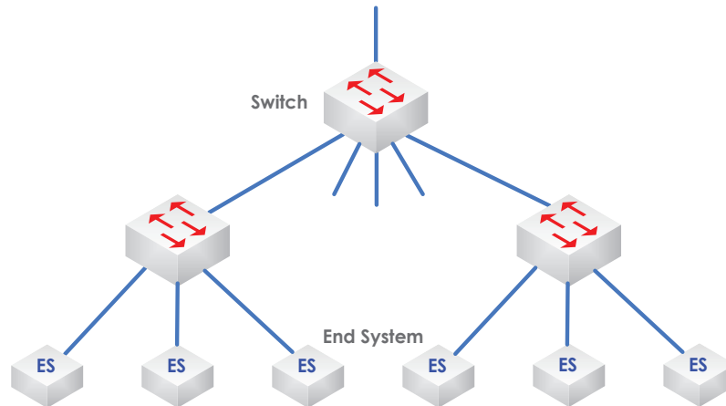
Figure 4-7: A TTE example network
