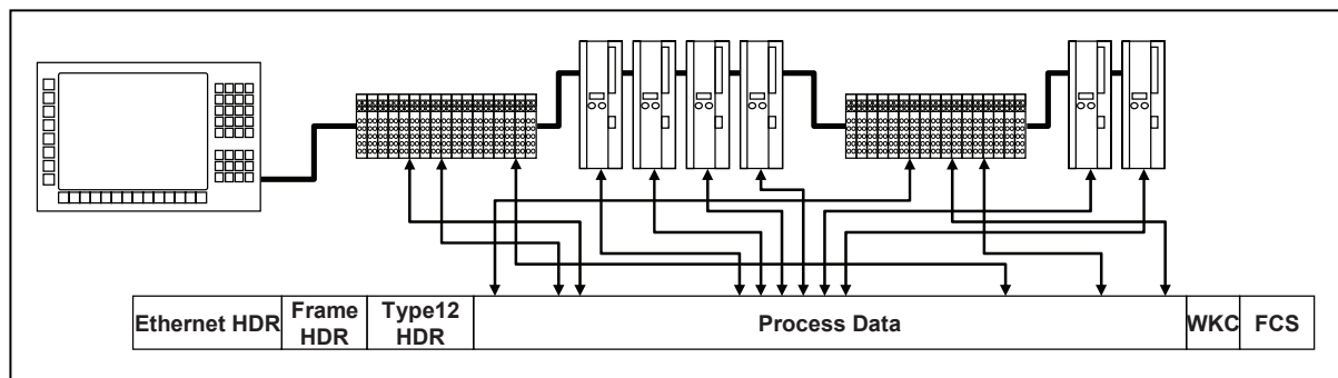
Figure 4 – Mapping of data in a frame
