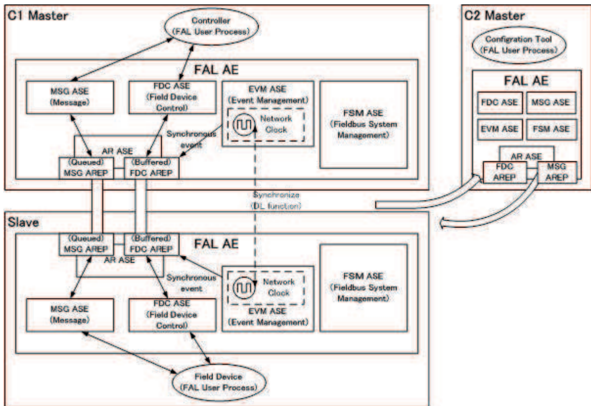
Figure 1 – FAL ASE model of Type 24
