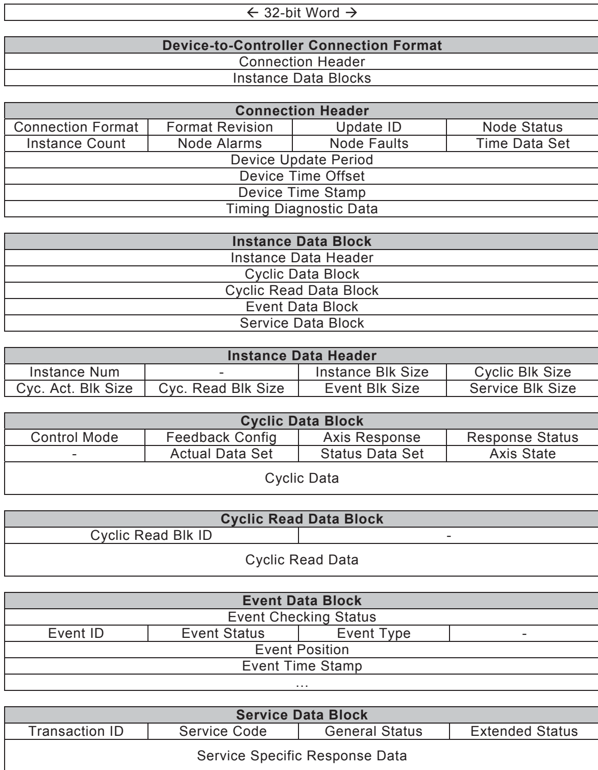
Figure 12 – Device-to-Controller Connection Format
