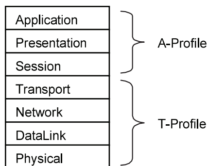
Figure 2 – OSI reference model and profiles
