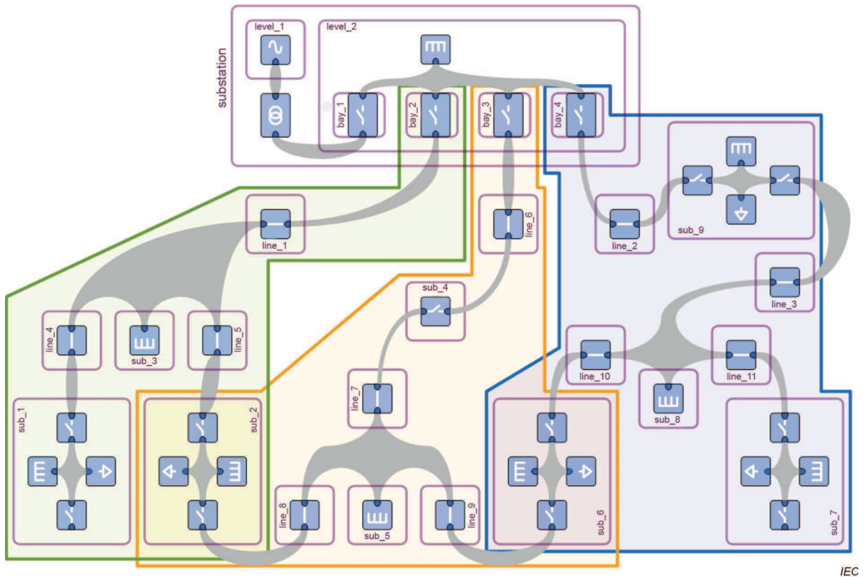
Figure 1 – Feeder containment principles
