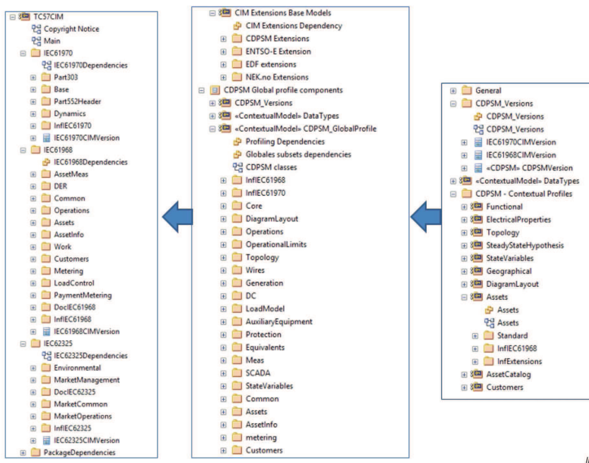
Figure 4 – UML CDPSM profiles (informative)
