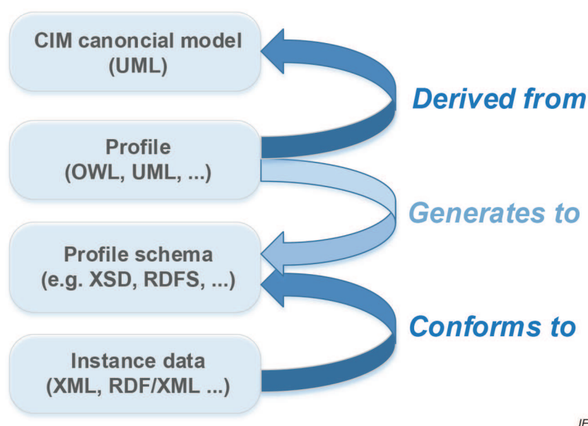
Figure 3 – Main steps for profiling CIM
