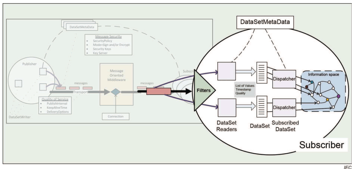
Figure 7 – Subscriber details
