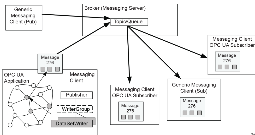
Figure 16 – Broker overview
