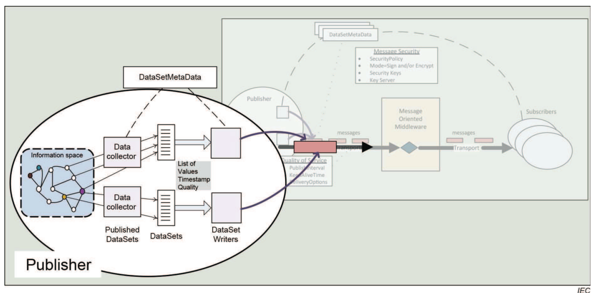
Figure 5 – Publisher details
