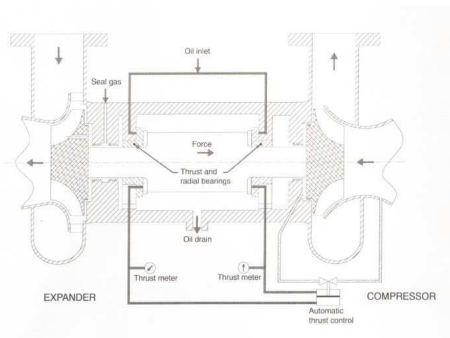
Figure 1 — Automatic thrust balancing system
