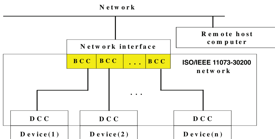
Figure 2—Connection topology with a remote host
