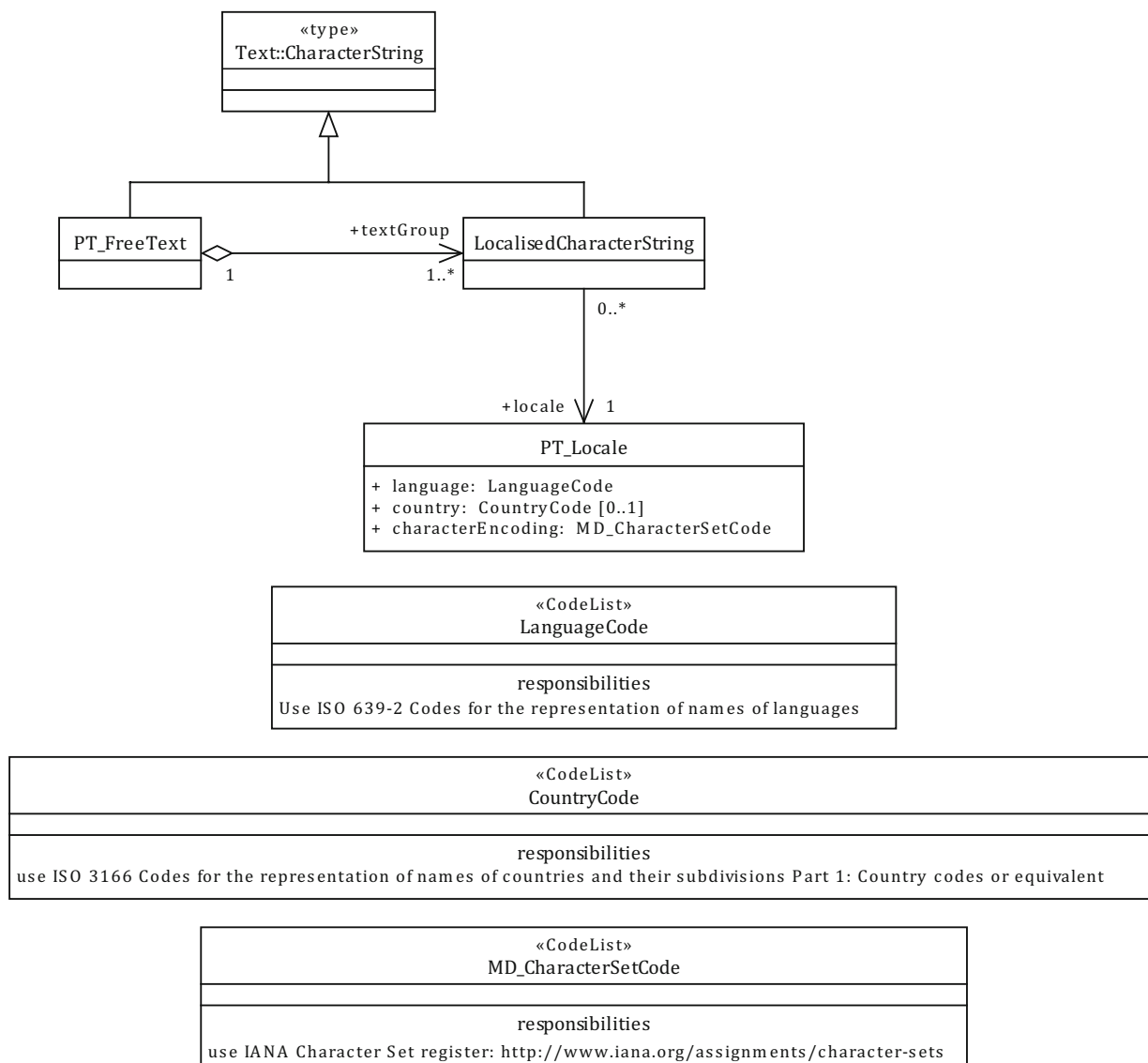
Figure 23 — PT_Locale schema
