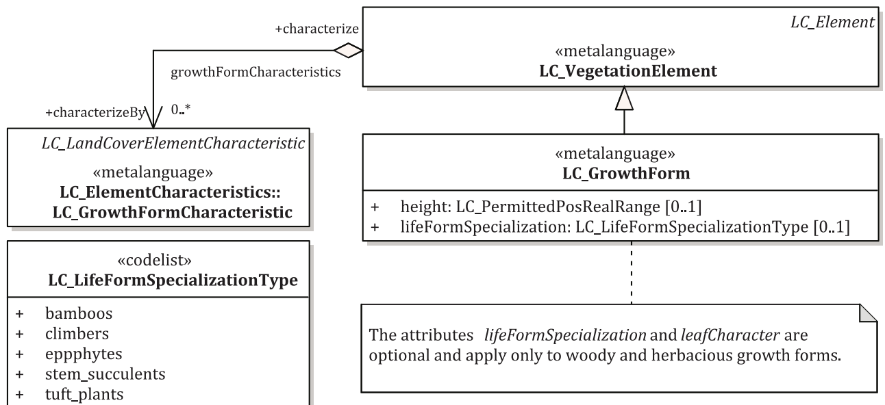
Figure 9 — Subtypes of LC_VegetationElement
