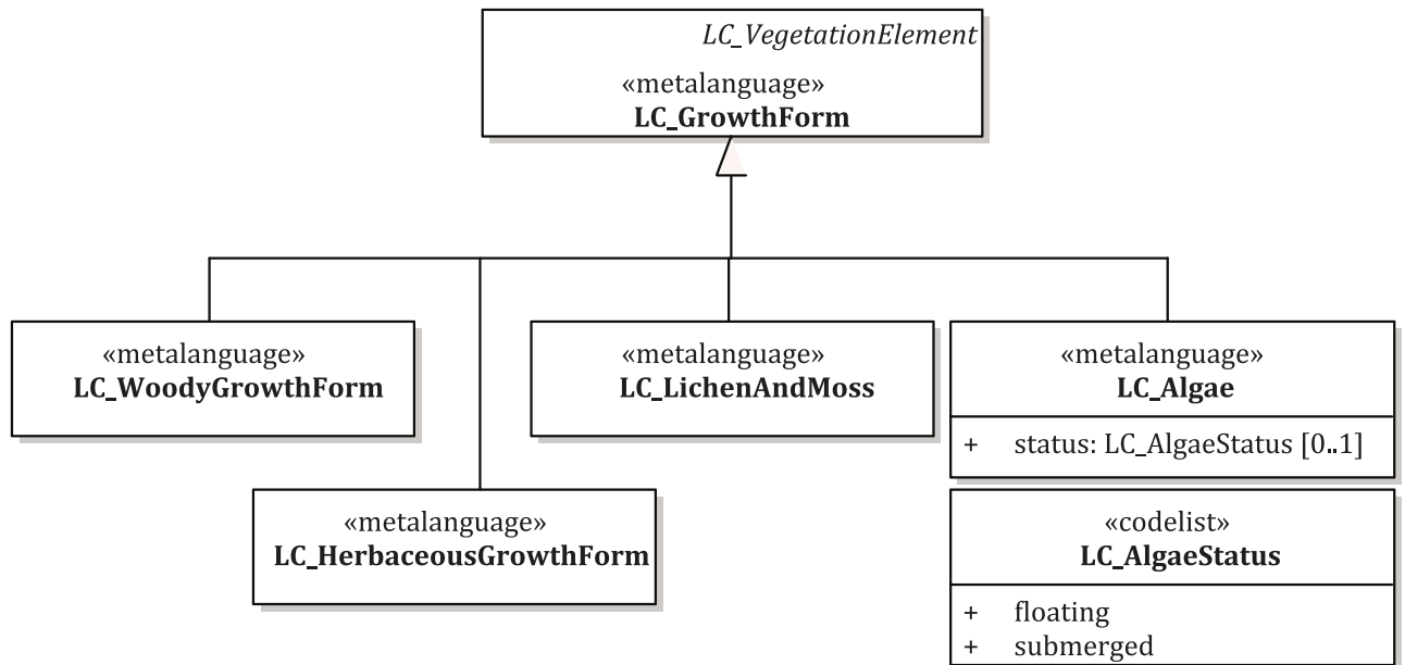
Figure 10 — Subtypes of LC_GrowthForm
