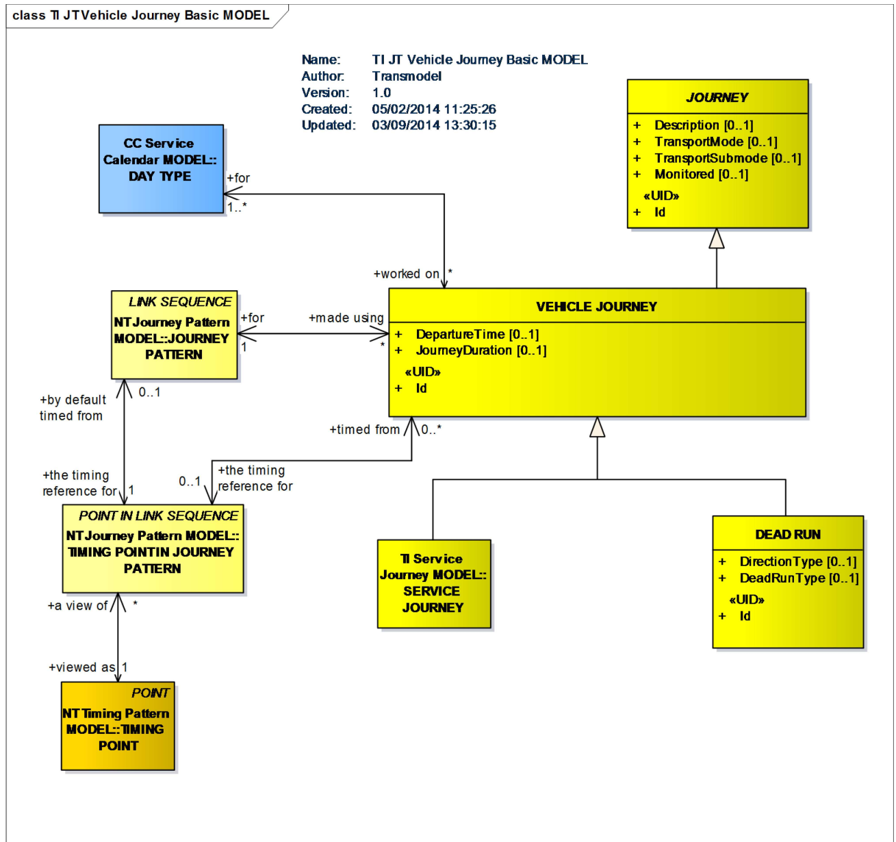
Figure 1 — Vehicle Journey – Basic Conceptual Model (UML)
