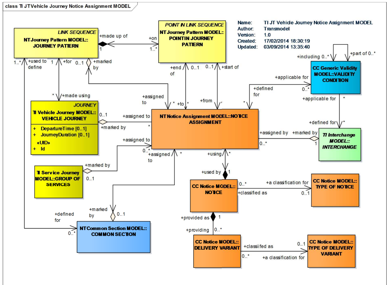
Figure 3 — Vehicle Journey Notice Assignment – Conceptual Model (UML)
