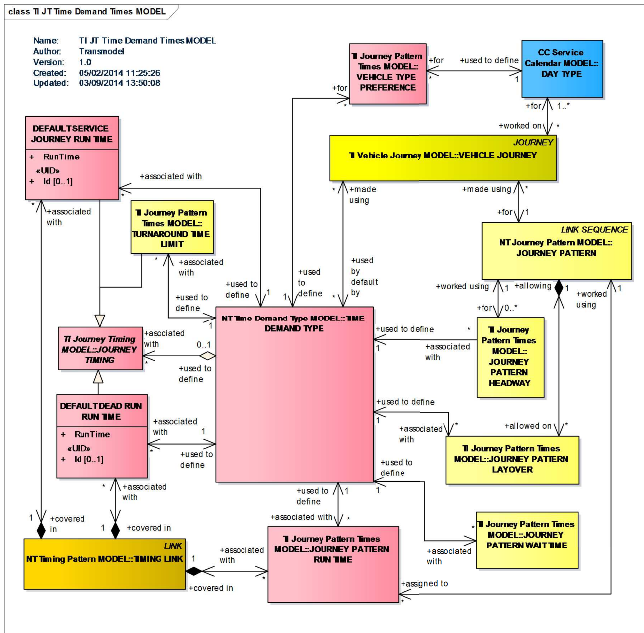
Figure 6 —Time Demand Times – Conceptual Model (UML)
