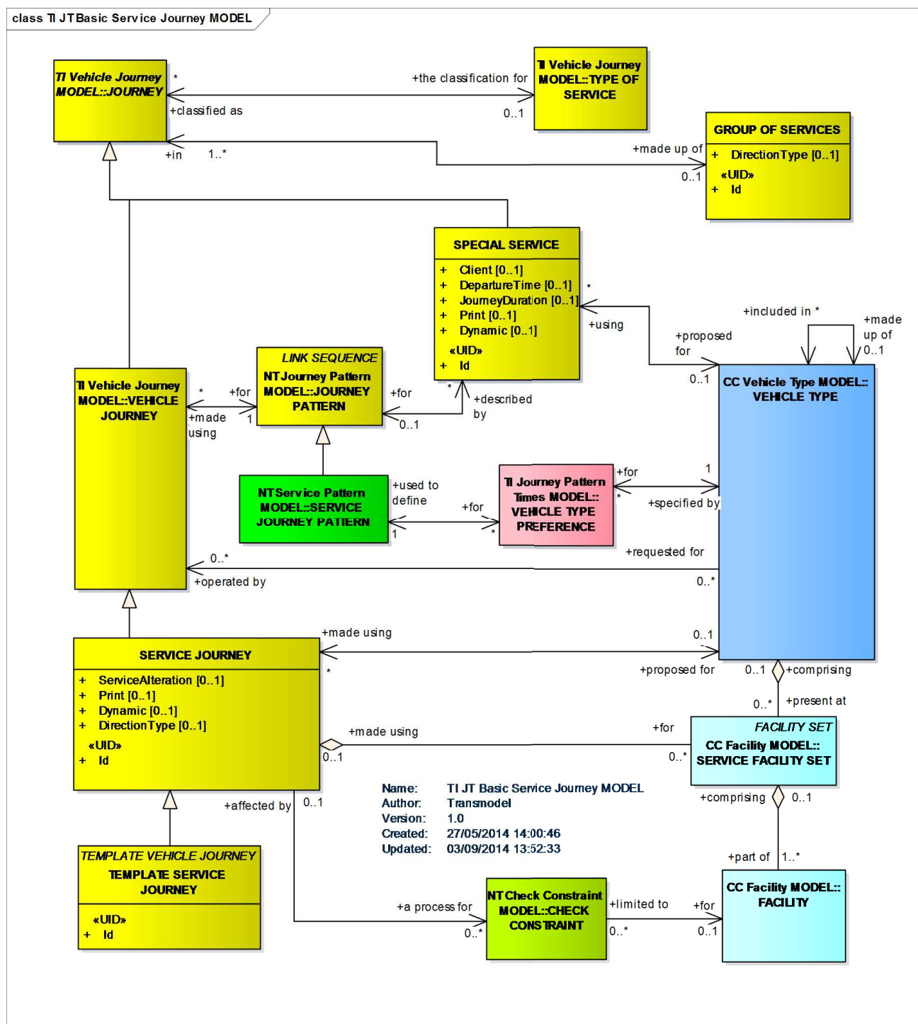
Figure 4 — Service Journey – Basic Conceptual Model (UML)
