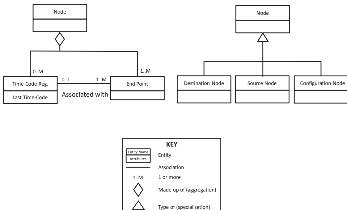
Figure 3-4: UML notation
