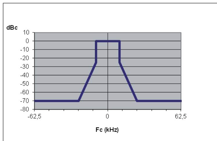
Figure 3 – Modulation spectrum for slotted transmission
