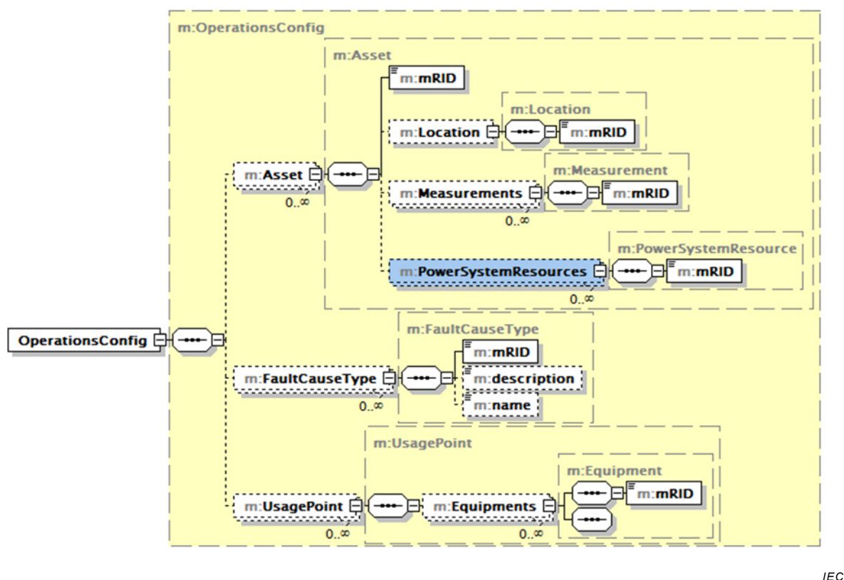
Figure 3 – OperationsConfiguration message payload
