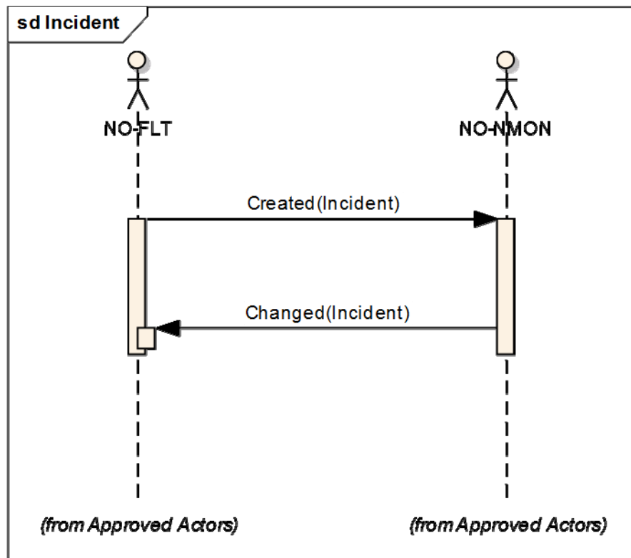
Figure 29 – Incident
