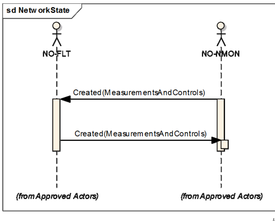
Figure 4 – MeasurementsAndControls
