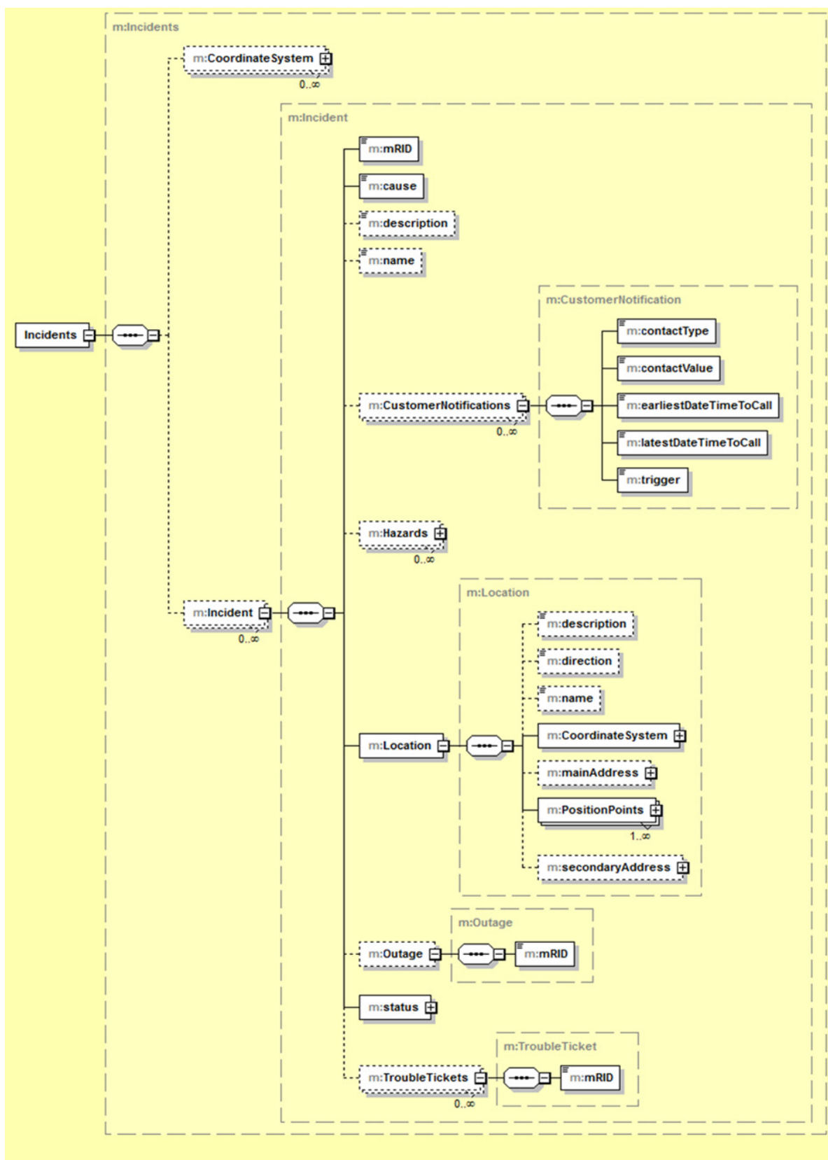
Figure 30 – Incident message payload
