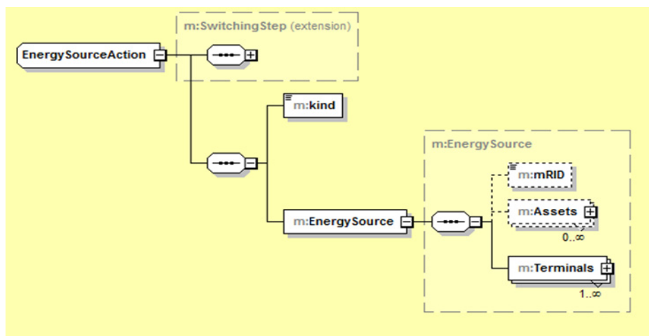
Figure 20 – SwitchingPlan message payload, EnergySourceAction detail
