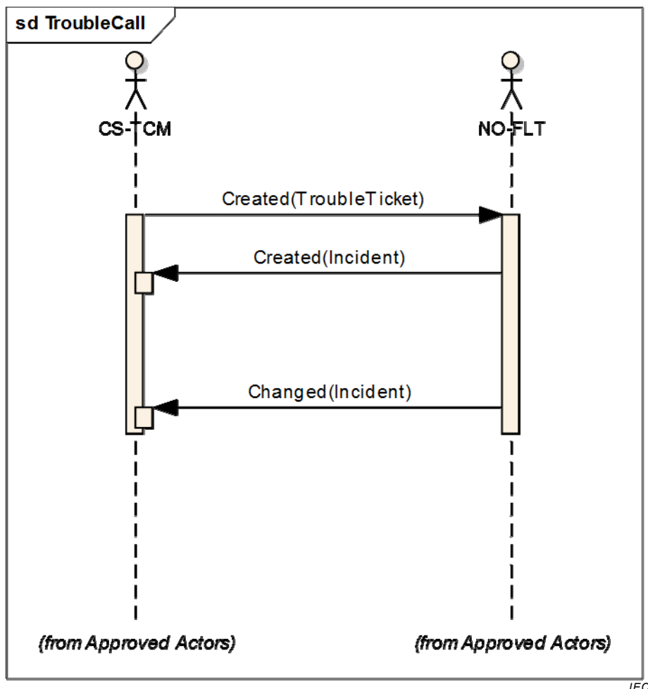
Figure 28 – Trouble Ticket
