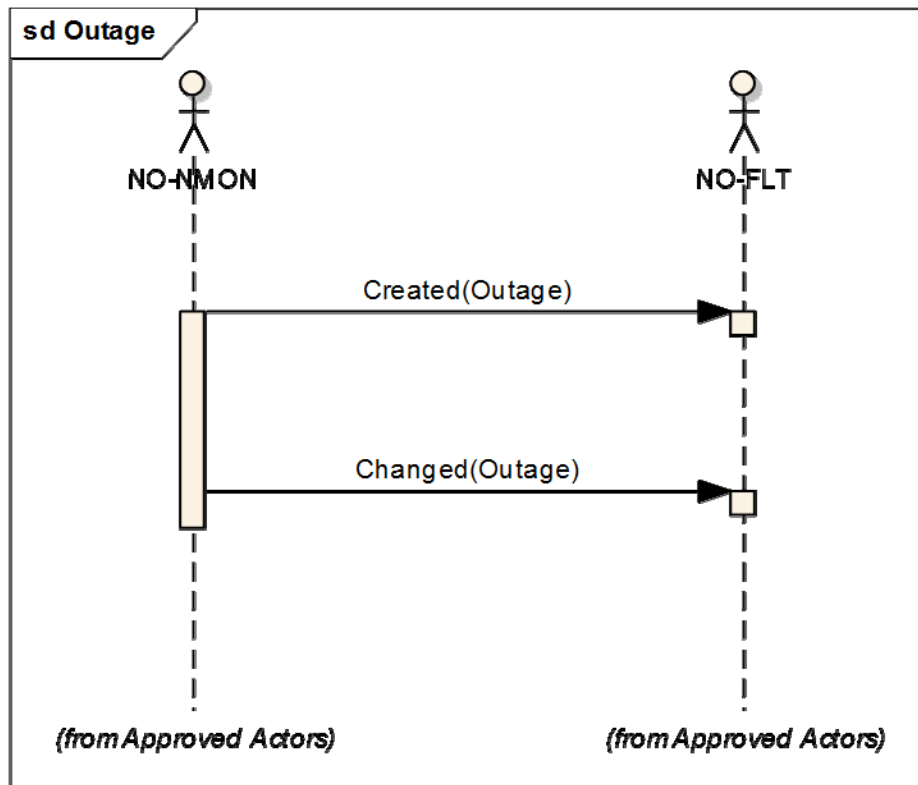
Figure 31 – Outage
