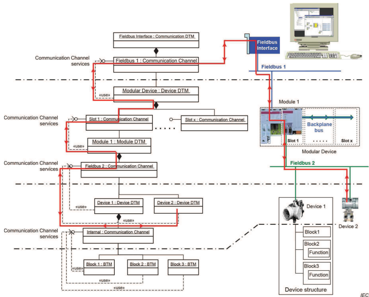
Figure 19 – Nested communication
