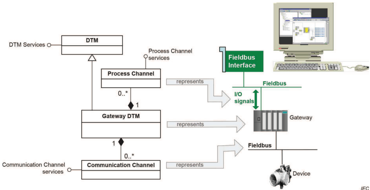
Figure 7 – Gateway DTM
