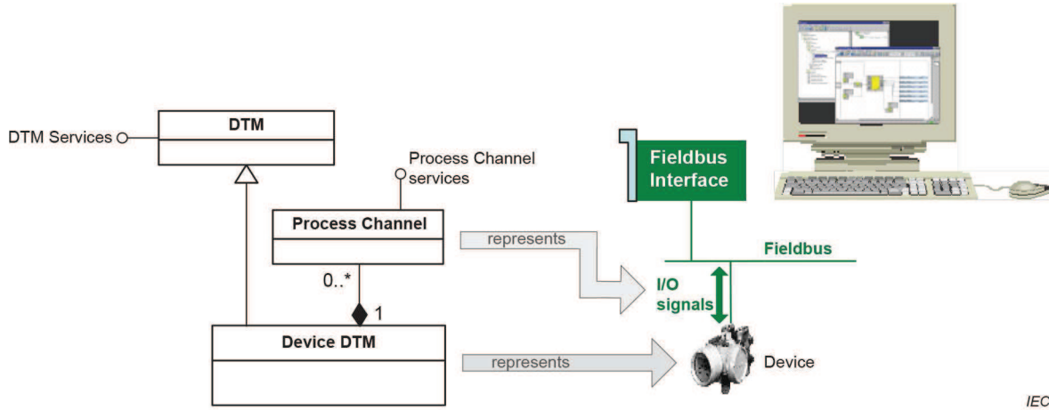
Figure 6 – Device DTM
