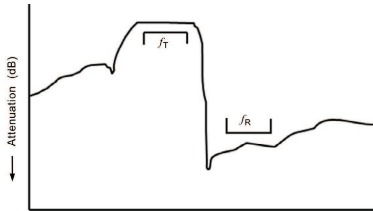
Figure 2 – Basic TX filter response example of SAW and BAW duplexers
