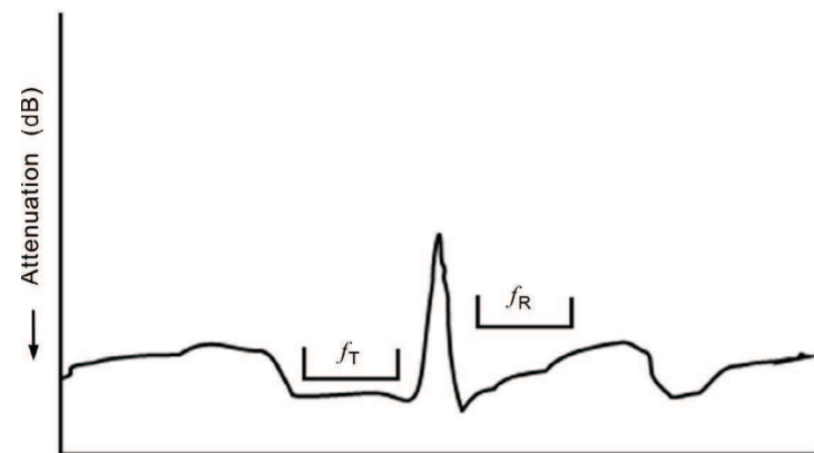
Figure 4 – Basic isolation characteristics example of SAW and BAW duplexers
