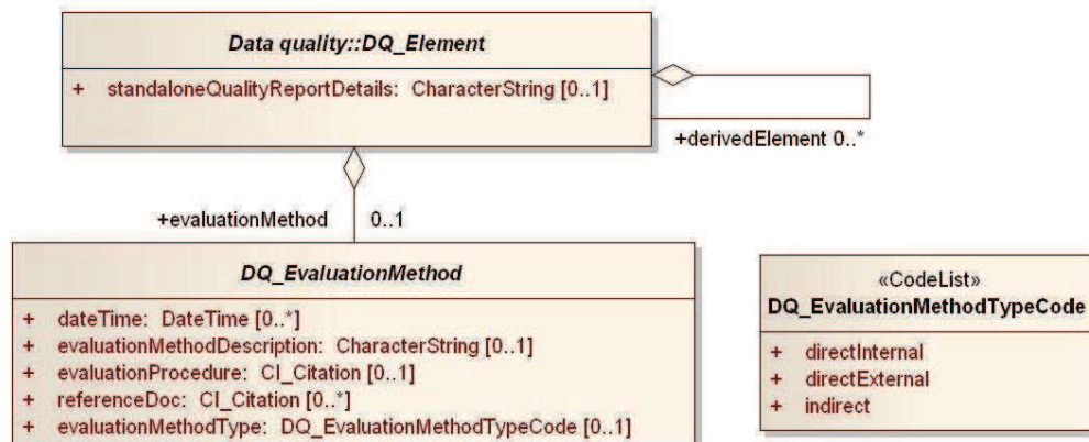
Figure 8 — Data quality evaluation method
