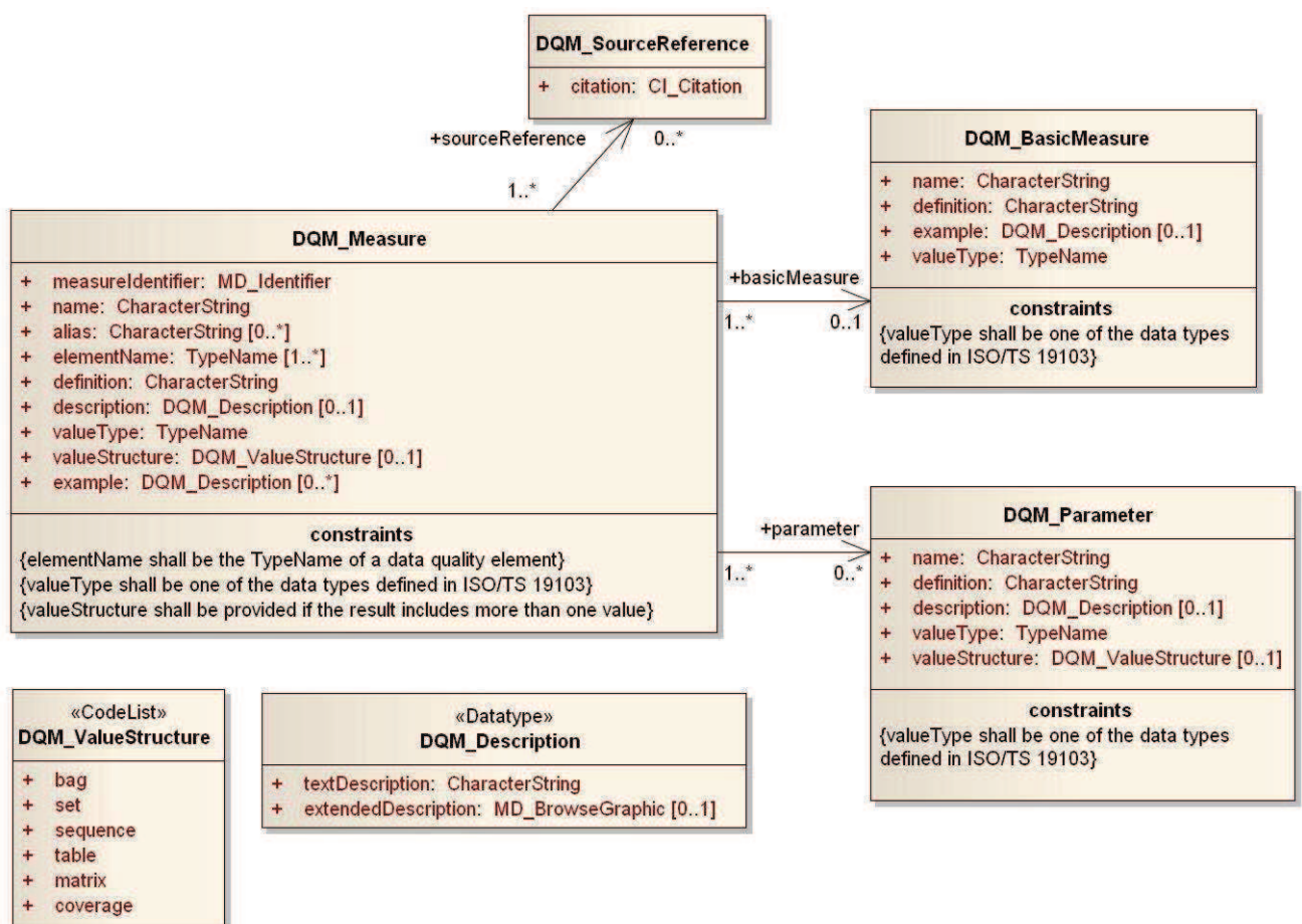
Figure 12 — Data quality measures
