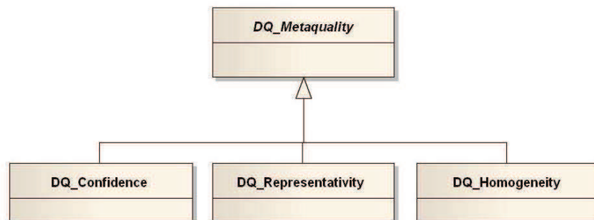
Figure 10 — Metaquality elements
