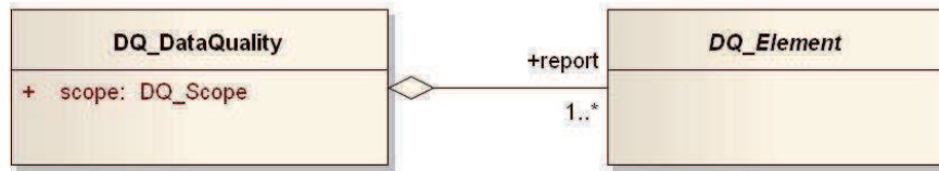
Figure 3 — Data quality unit
