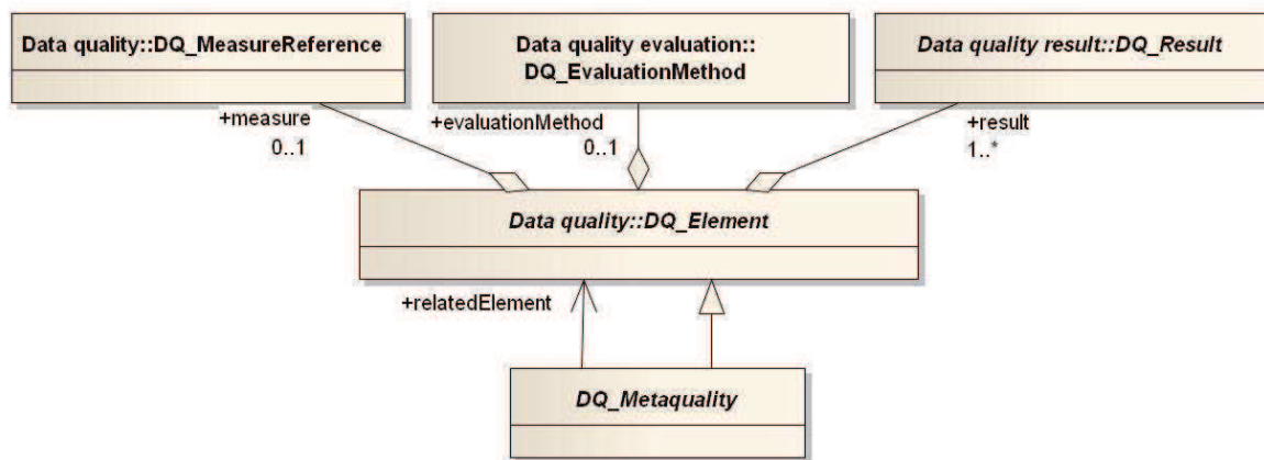
Figure 11 — Metaquality descriptors
