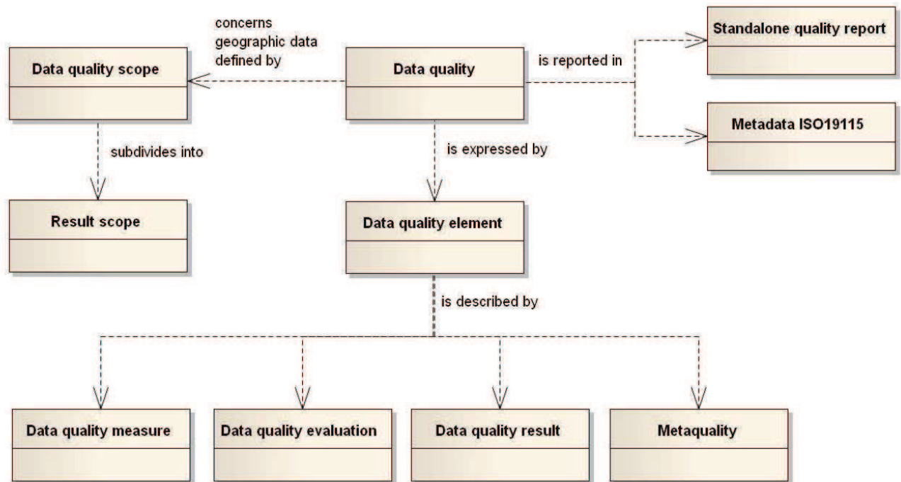
Figure 1 — Conceptual model on quality for geographic data
