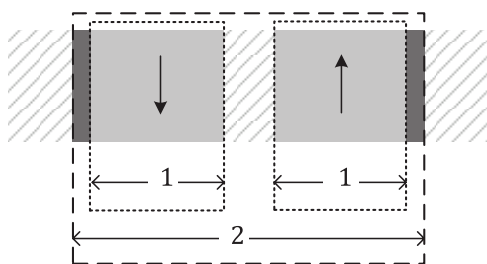
c) Single carriageway with sidewalk (1 RoadBelt & 2 RoadBeltElements)
