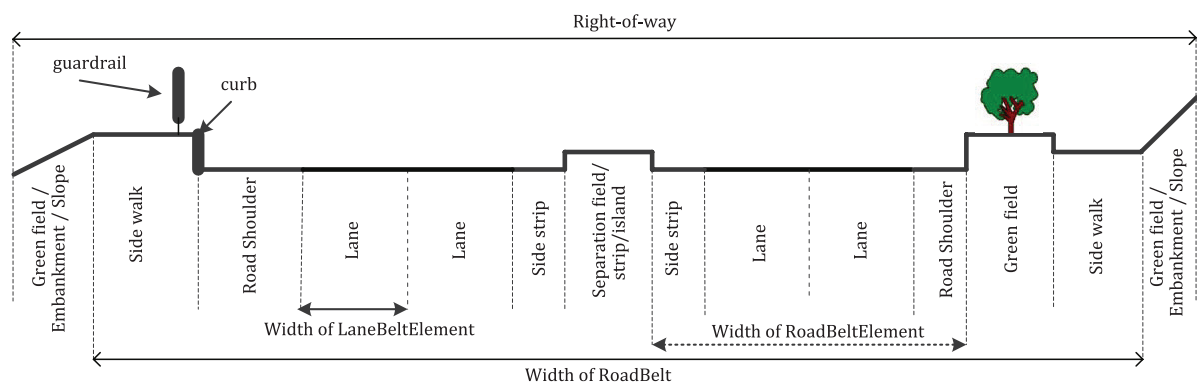
Figure 30 — Typical cross-section of road structure
