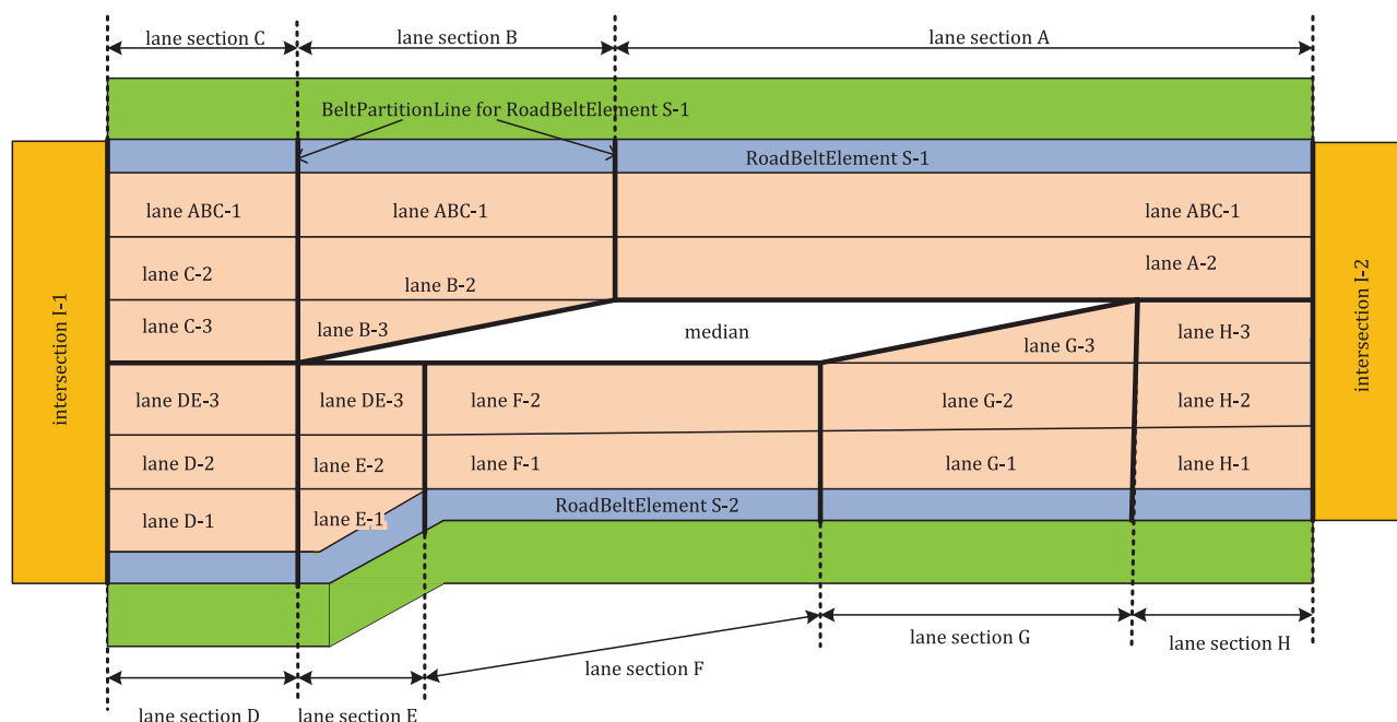
Figure 32 — Example of lane structure in RoadBeltElement
