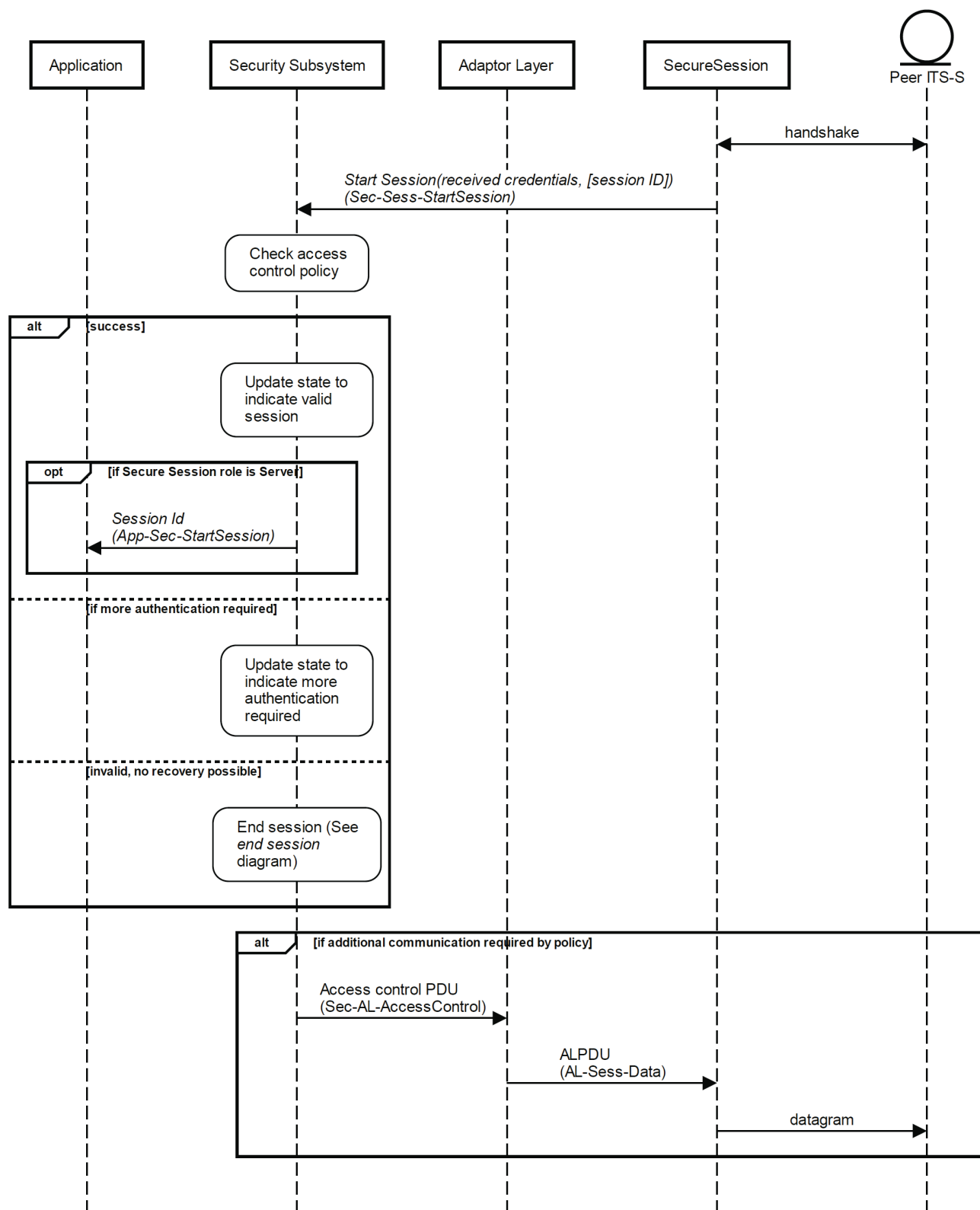
Figure 13 — Sequence diagram for Start Session
