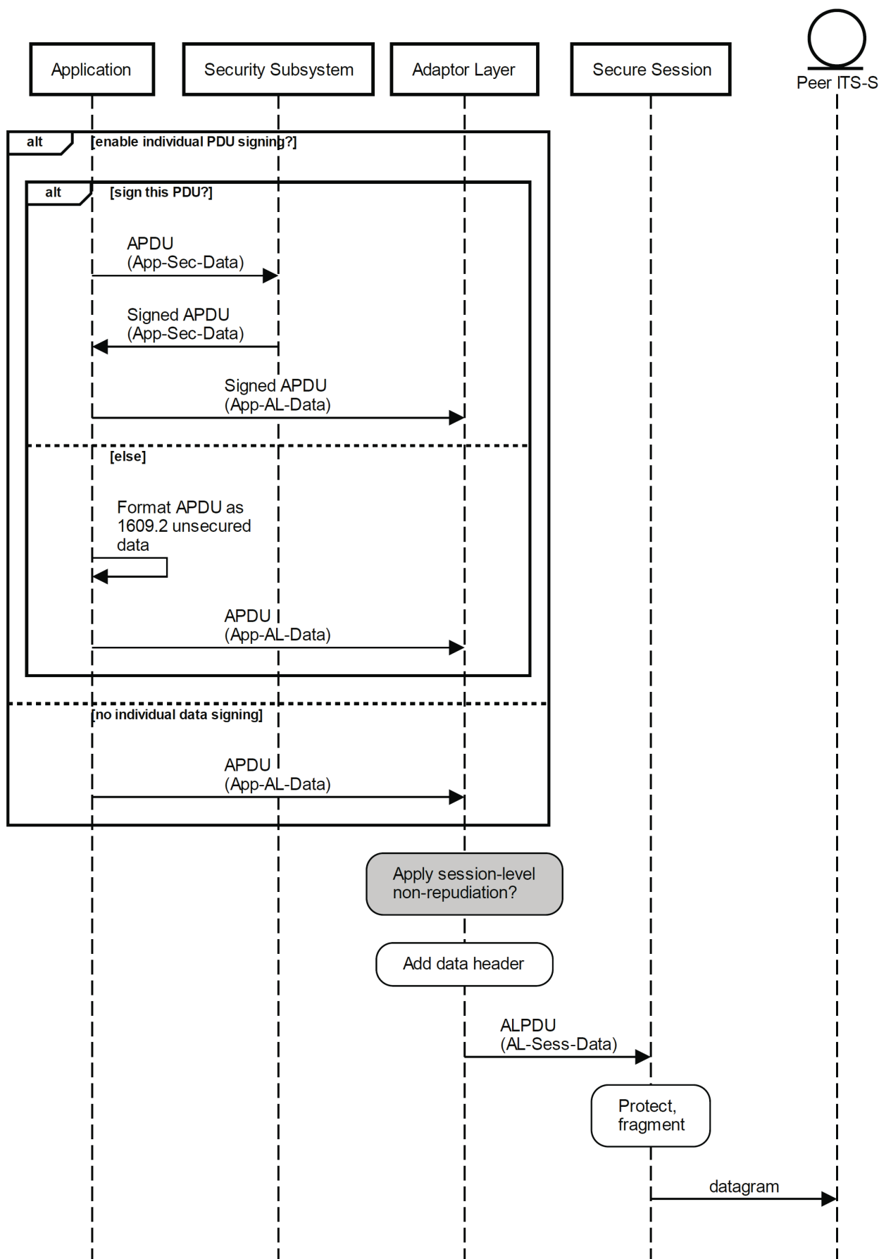
Figure 14 — Sequence diagram for sending data
