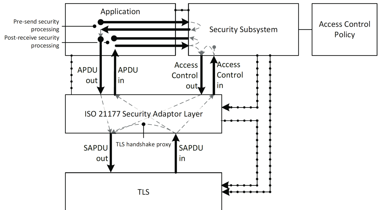
Figure 9 — Interactions between local functional elements
