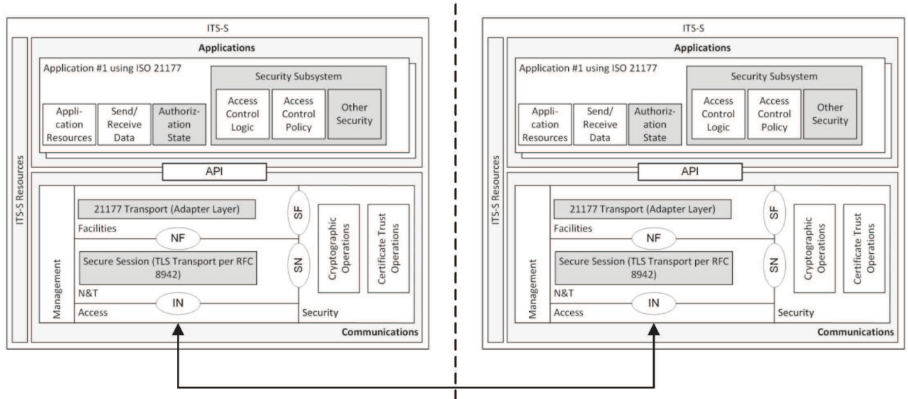
Figure 7 — Logical Architecture with two ITS-SUs
