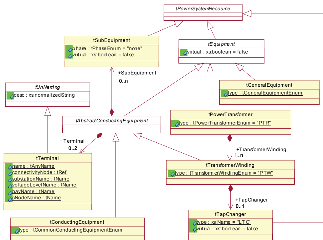
Figure 11 – UML diagram for equipment type inheritance and relations
