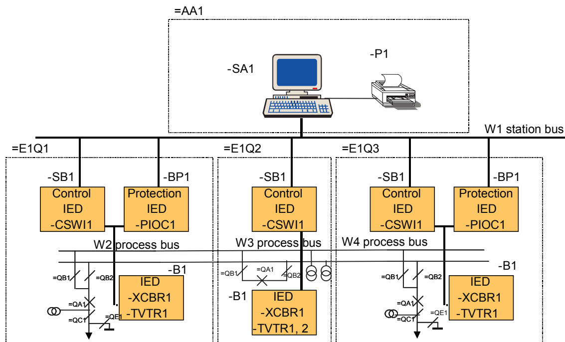
Figure 3 – SA system configuration example
