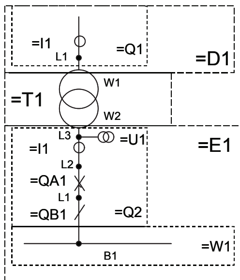
Figure 12 - Substation section example
