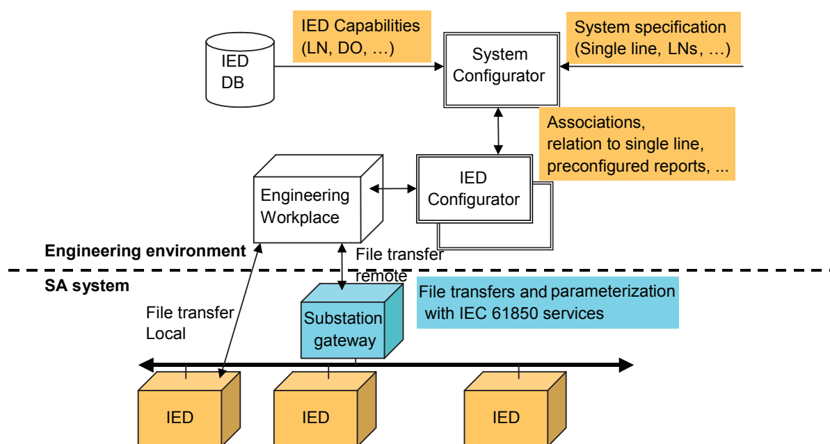
Figure 1 – Reference model for information flow in the configuration process
