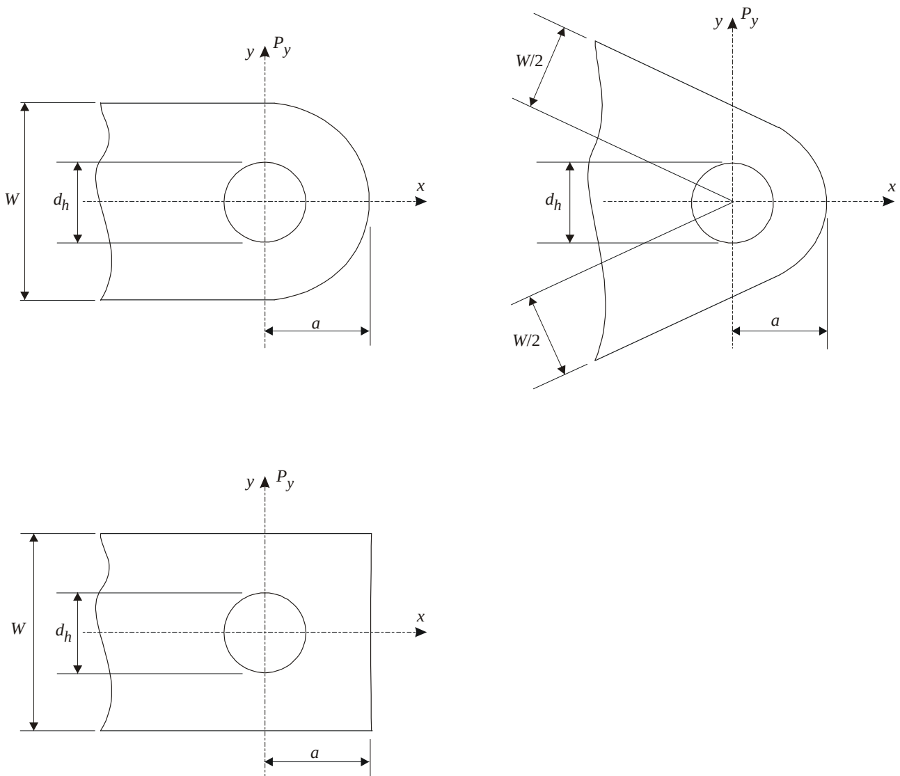
Sketch 1.1 General lug geometry and loading
